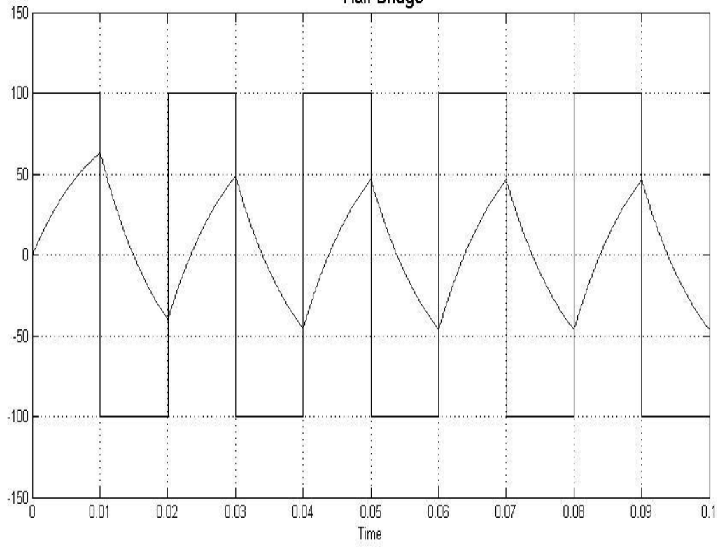
Half Bridge
